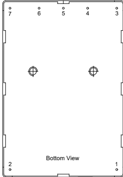
Pin Connections
