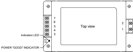
Pin Connections
